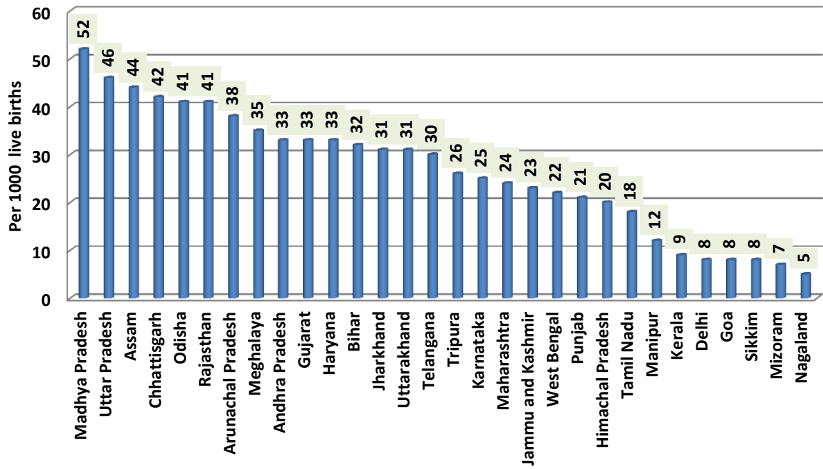
Fig. 1.1: Infant Mortality Rate in Rural Areas - State-wise
